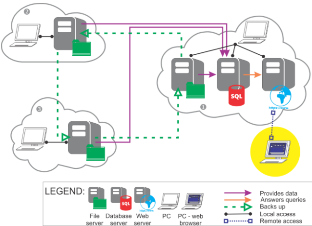
Figure 1. A schematic drawing of dependencies and data flow in a multidisciplinary database system
